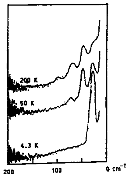
Fig. 4. Inelastic neutron scattering spectrum of [\text{Cr}_3\text{O}(\text{OAc})_6(\text{H}_2\text{O})_3]\text{Cl} \cdot 5\text{H}_2\text{O} (from ref. 8).
